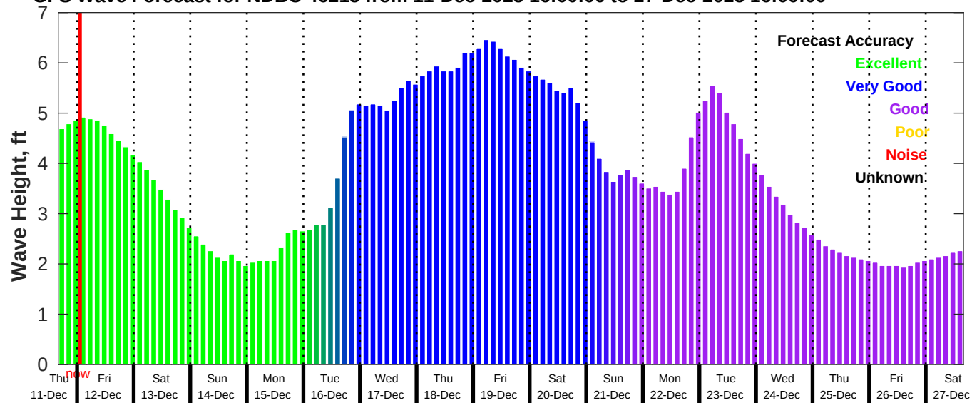
GFS Wave Forecast for NDBC 46215 from 11-Dec-2025 16:00:00 to 27-Dec-2025 16:00:00
