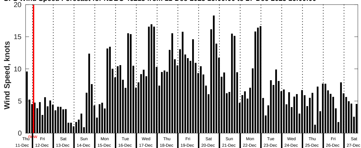
GFS Wind Speed Forecast for NDBC 46215 from 11-Dec-2025 16:00:00 to 27-Dec-2025 16:00:00
