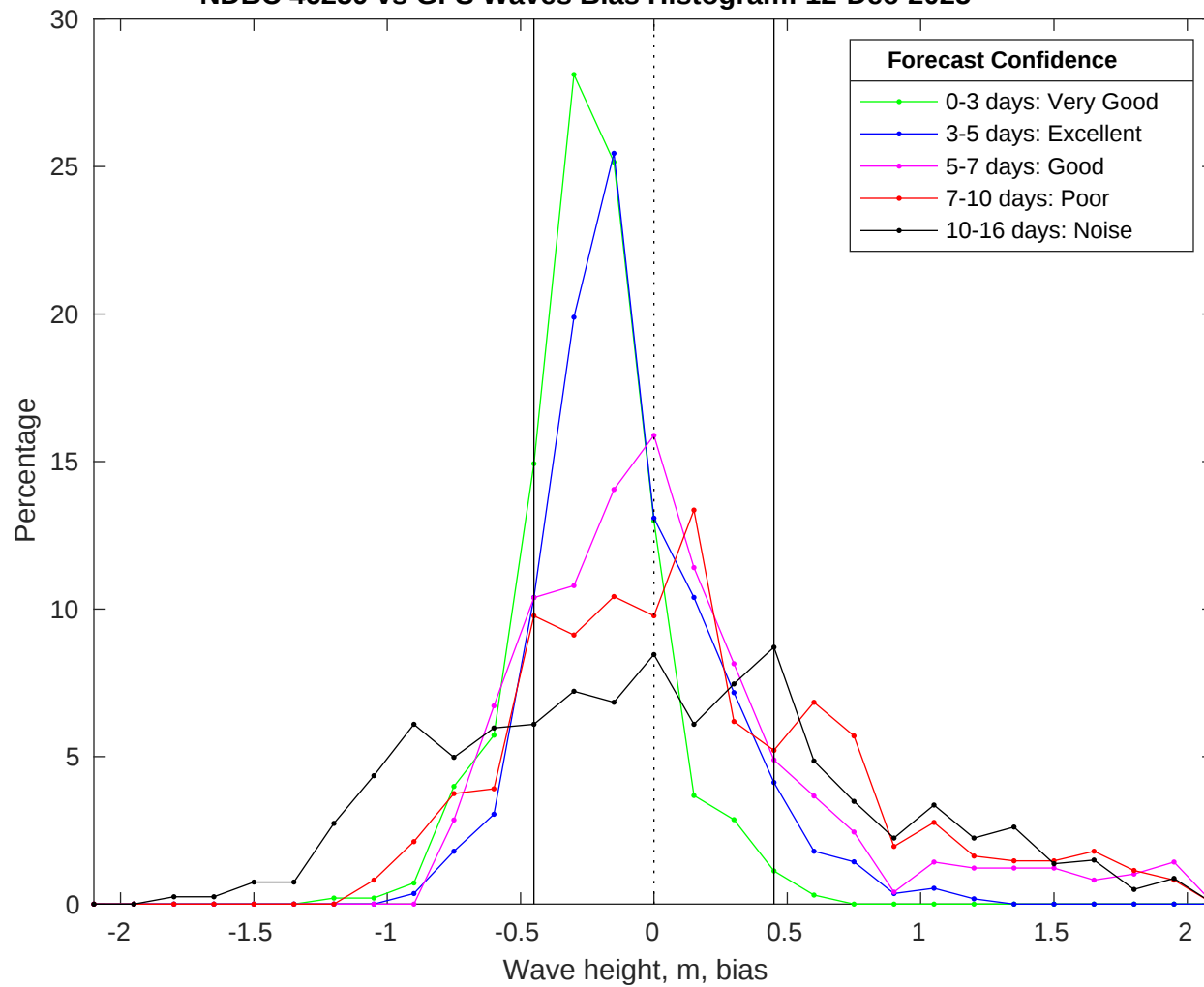
NDBC 46259 vs GFS Waves Bias Histogram: 12-Dec-2025
