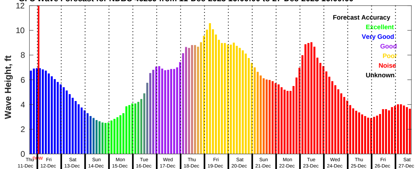
GFS Wave Forecast for NDBC 46259 from 11-Dec-2025 16:00:00 to 27-Dec-2025 16:00:00
