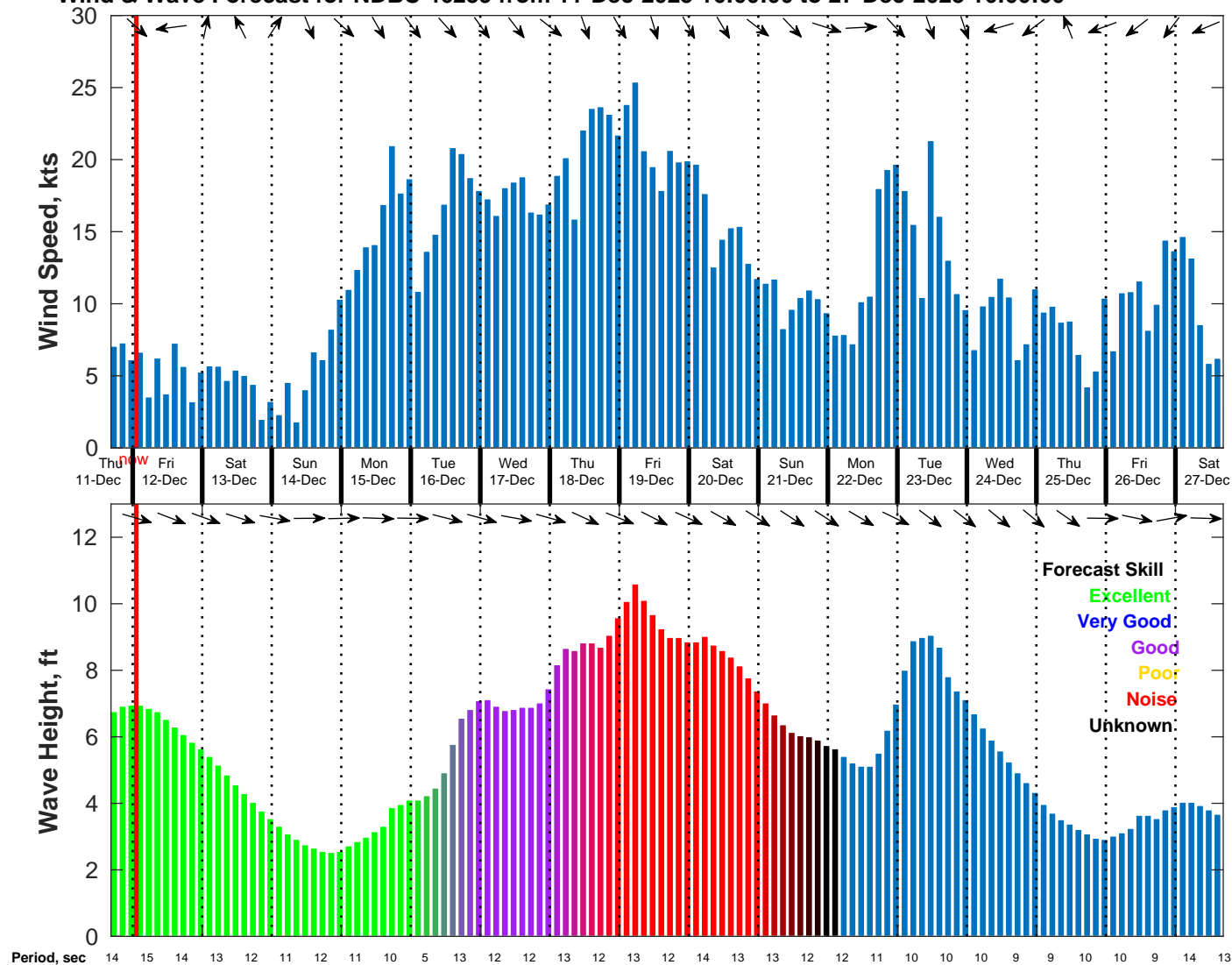
Wind & Wave Forecast for NDBC 46259 from 11-Dec-2025 16:00:00 to 27-Dec-2025 16:00:00
