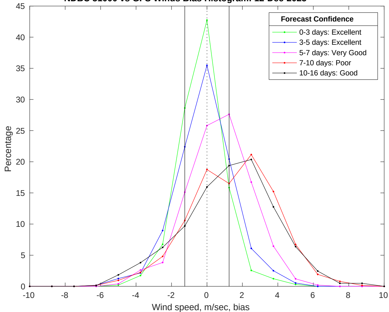
NDBC 51000 vs GFS Winds Bias Histogram: 12-Dec-2025
