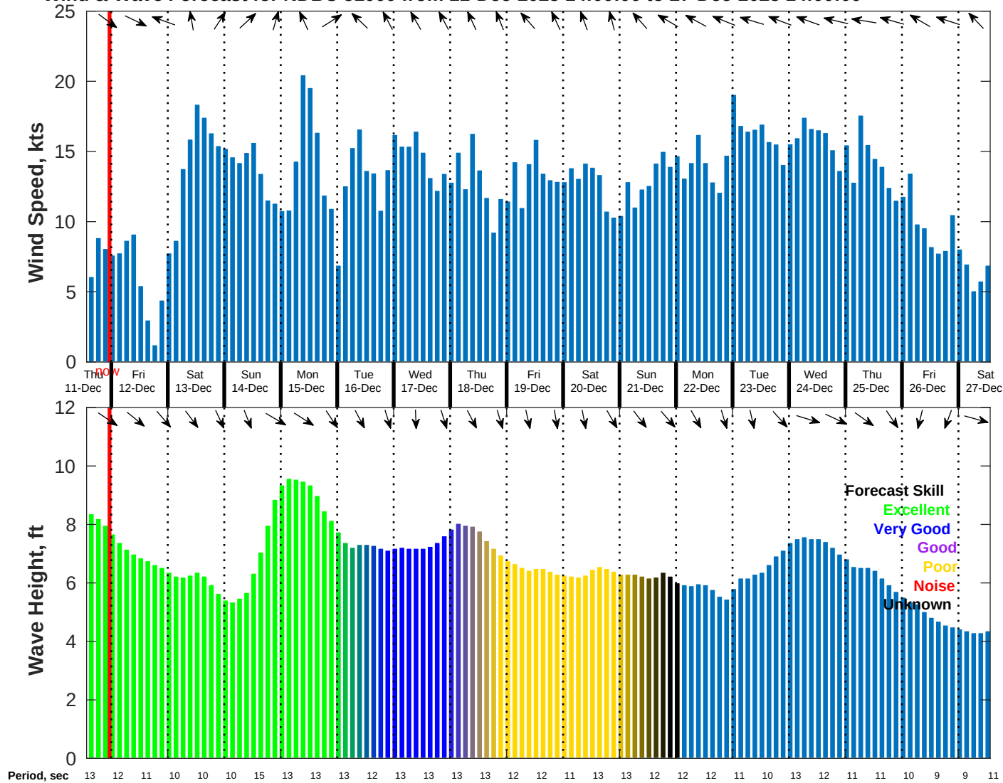
Wind & Wave Forecast for NDBC 51000 from 11-Dec-2025 14:00:00 to 27-Dec-2025 14:00:00
