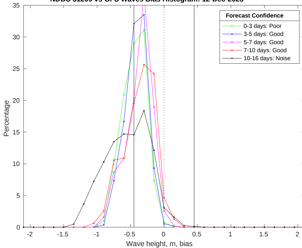
NDBC 51209 vs GFS Waves Bias Histogram: 12-Dec-2025
