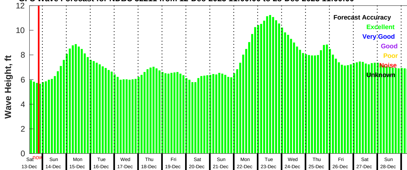
GFS Wave Forecast for NDBC 52211 from 12-Dec-2025 11:00:00 to 28-Dec-2025 11:00:00
