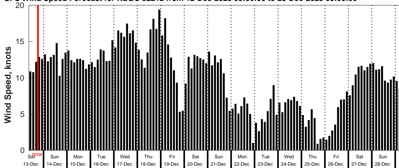
GFS Wind Speed Forecast for NDBC 52212 from 12-Dec-2025 09:00:00 to 28-Dec-2025 09:00:00
