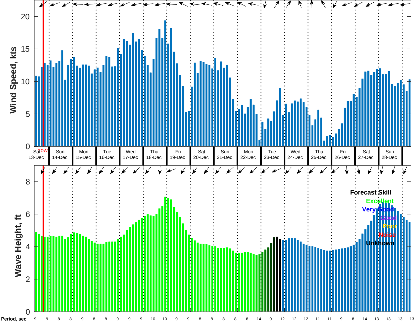
Wind & Wave Forecast for NDBC 52212 from 12-Dec-2025 09:00:00 to 28-Dec-2025 09:00:00
