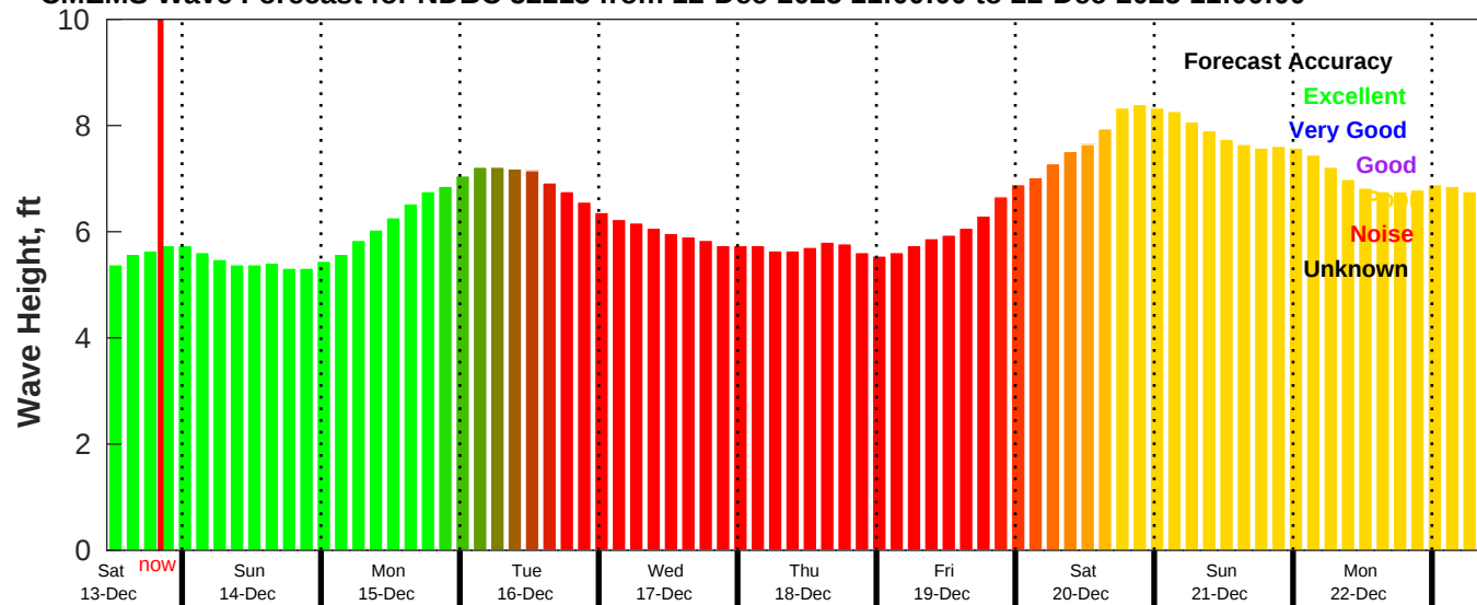
CMEMS Wave Forecast for NDBC 52213 from 12-Dec-2025 11:00:00 to 22-Dec-2025 11:00:00
