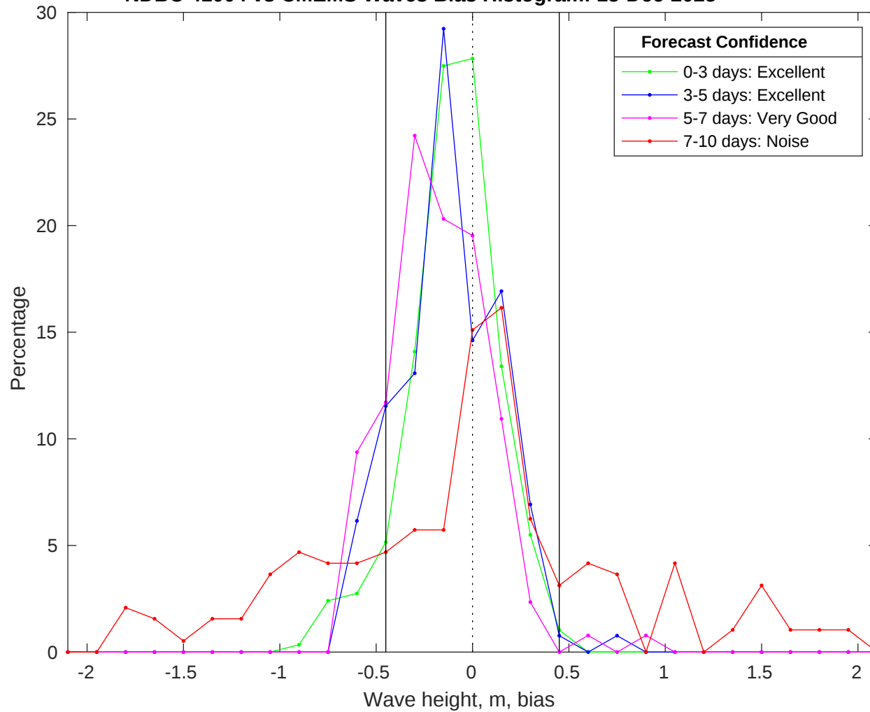
NDBC 41004 vs CMEMS Waves Bias Histogram: 13-Dec-2025
