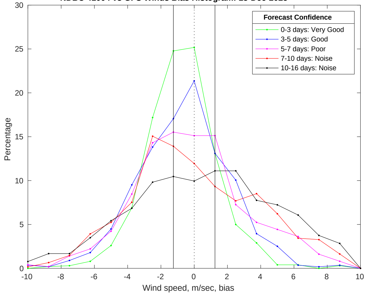
NDBC 41004 vs GFS Winds Bias Histogram: 13-Dec-2025
