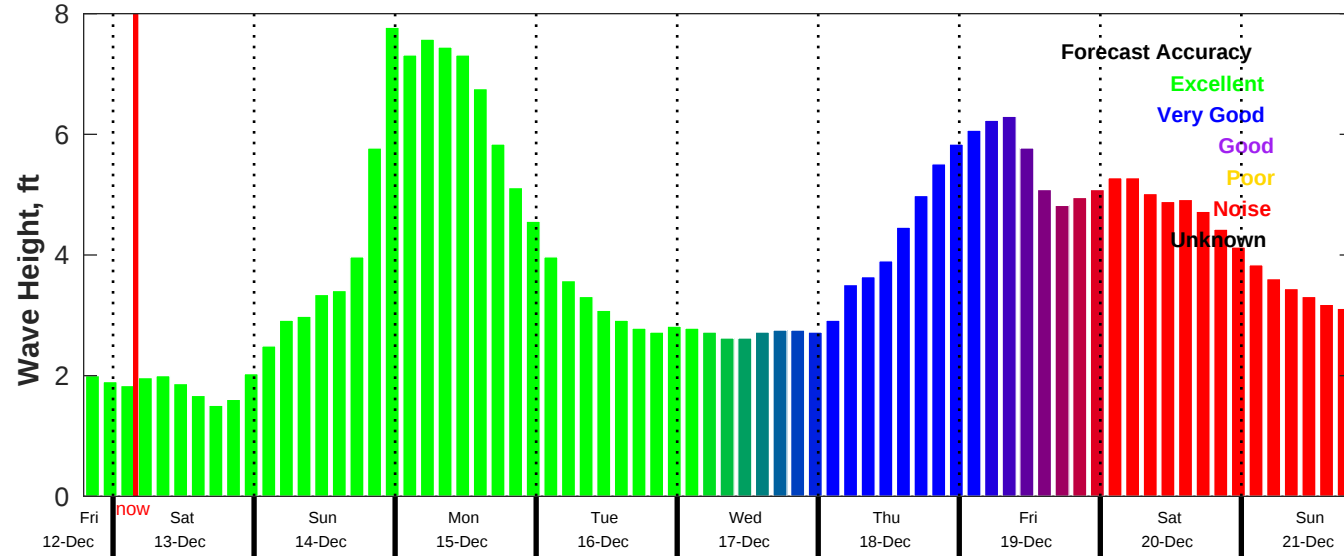
CMEMS Wave Forecast for NDBC 41004 from 12-Dec-2025 19:00:00 to 21-Dec-2025 19:00:00
