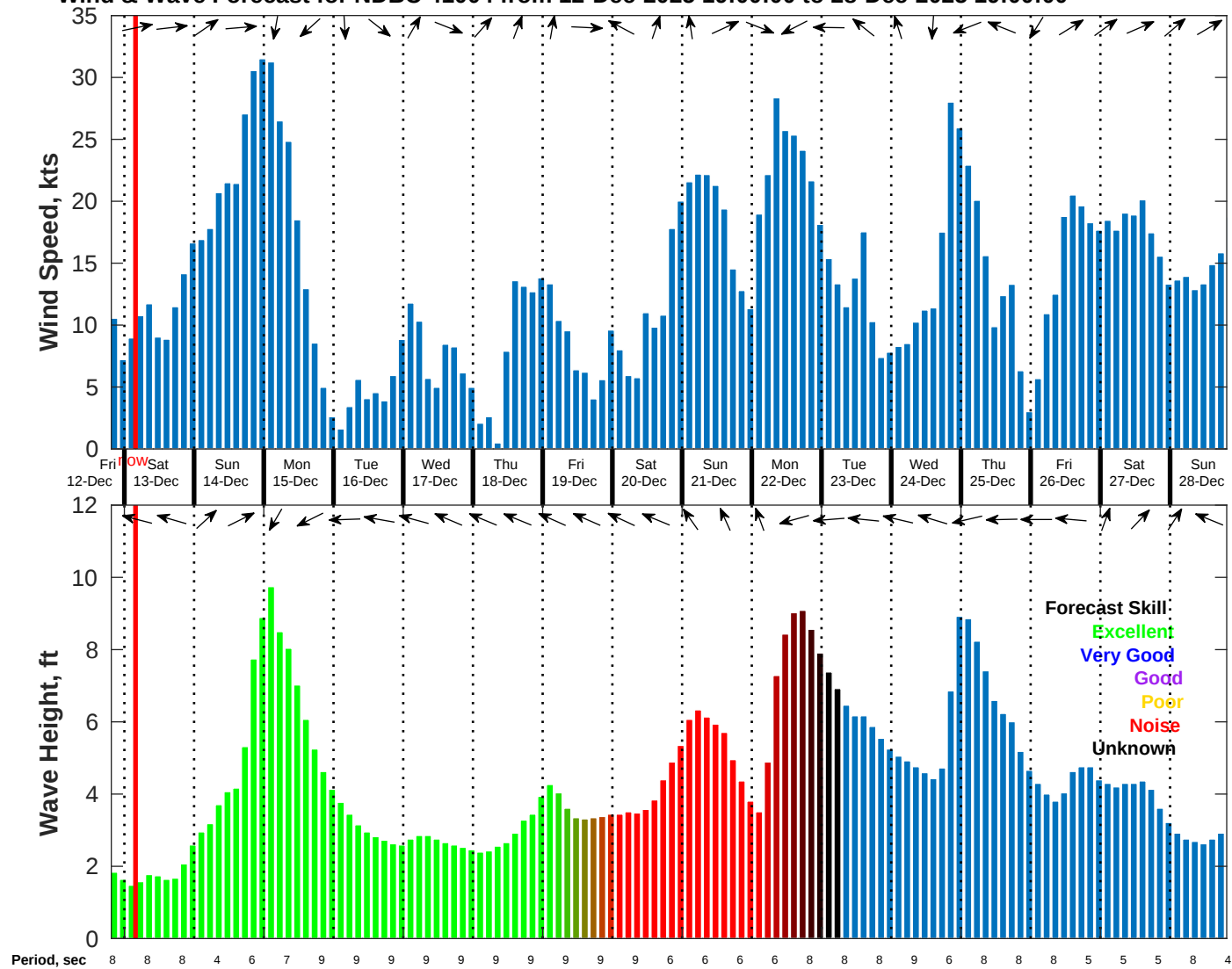
Wind & Wave Forecast for NDBC 41004 from 12-Dec-2025 19:00:00 to 28-Dec-2025 19:00:00
