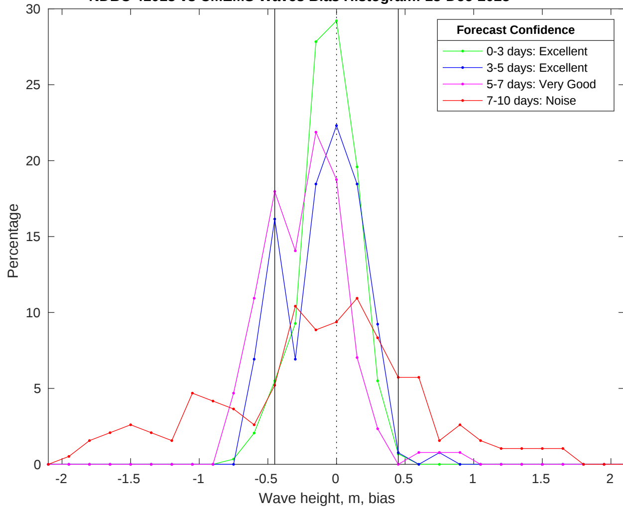
NDBC 41013 vs CMEMS Waves Bias Histogram: 13-Dec-2025
