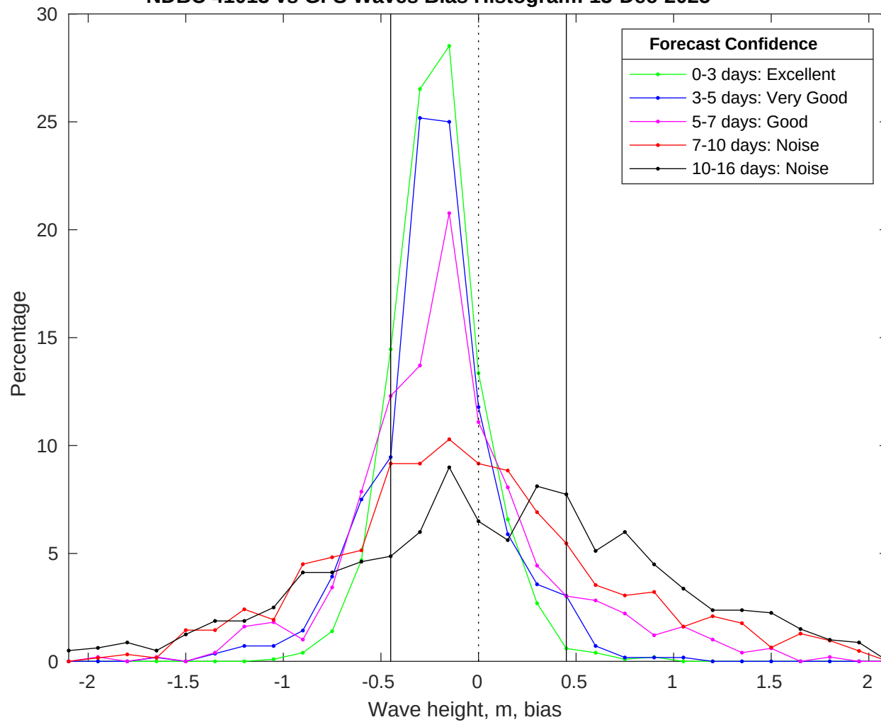
NDBC 41013 vs GFS Waves Bias Histogram: 13-Dec-2025
