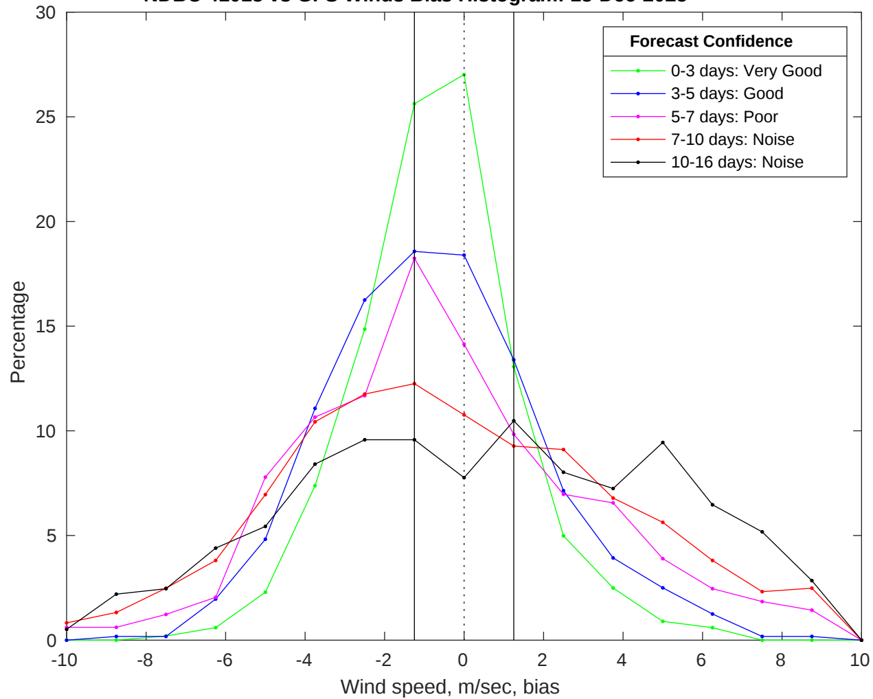
NDBC 41013 vs GFS Winds Bias Histogram: 13-Dec-2025
