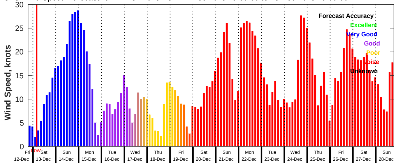
GFS Wind Speed Forecast for NDBC 41013 from 12-Dec-2025 19:00:00 to 28-Dec-2025 19:00:00
