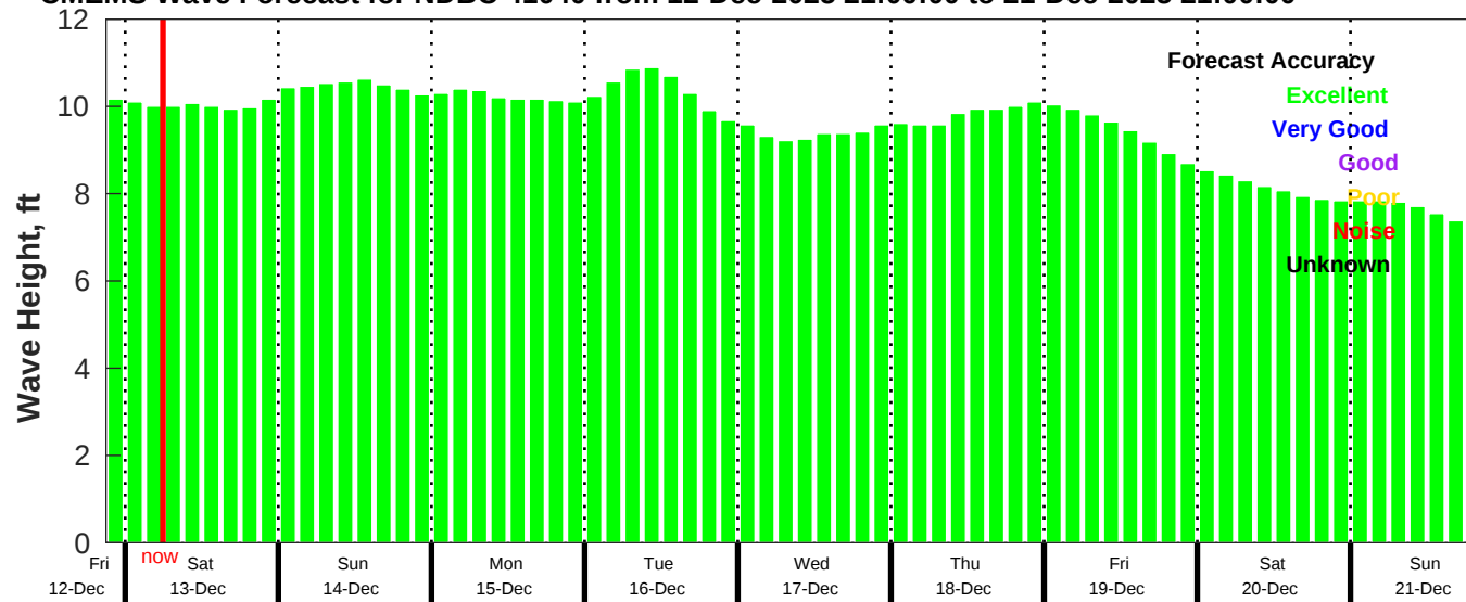
CMEMS Wave Forecast for NDBC 41040 from 12-Dec-2025 21:00:00 to 21-Dec-2025 21:00:00
