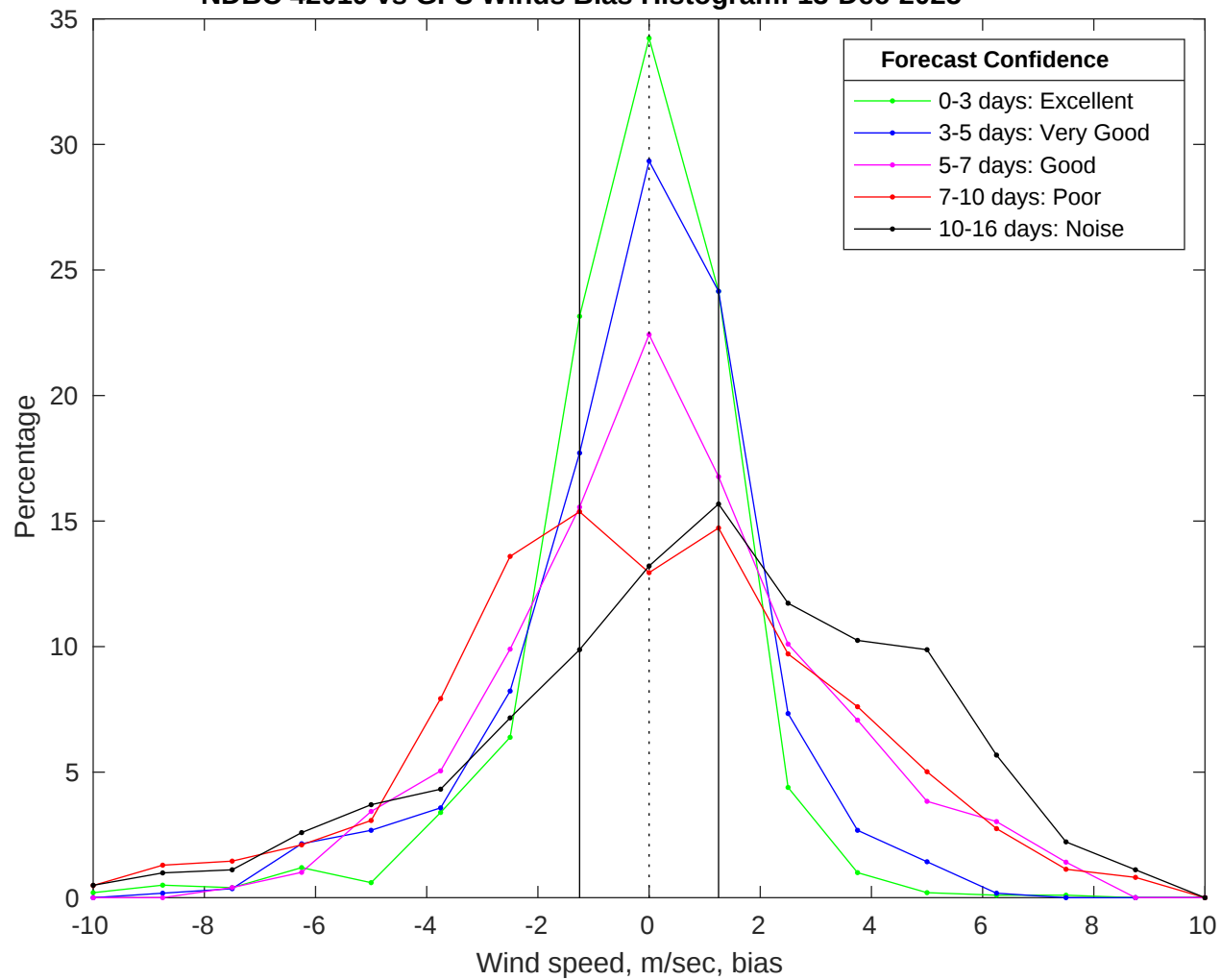
NDBC 42019 vs GFS Winds Bias Histogram: 13-Dec-2025
