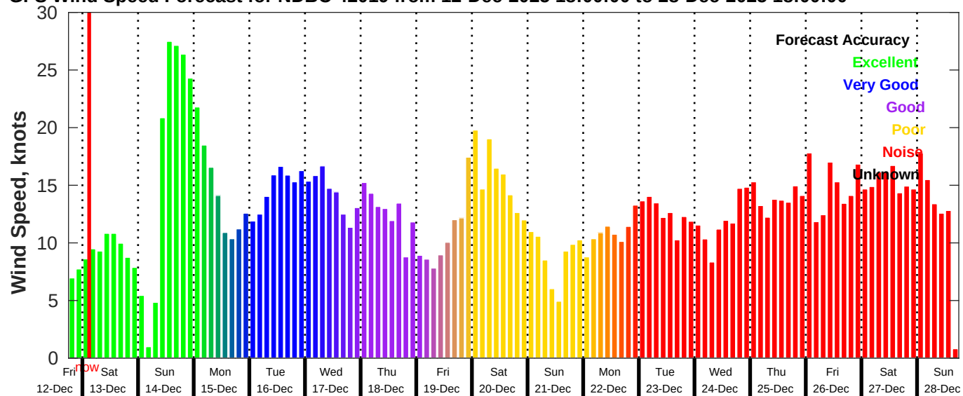
GFS Wind Speed Forecast for NDBC 42019 from 12-Dec-2025 18:00:00 to 28-Dec-2025 18:00:00
