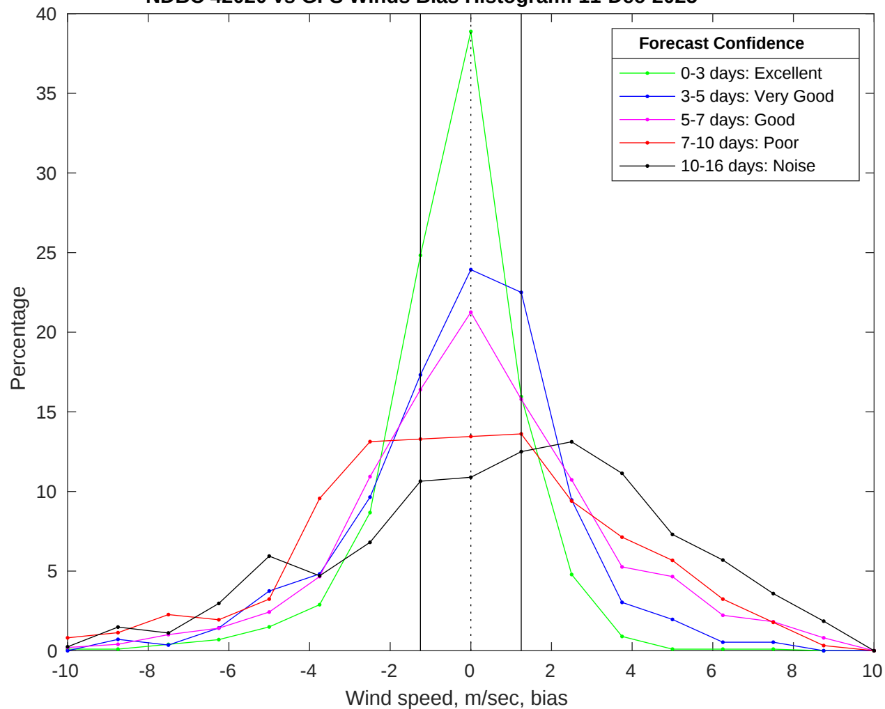
NDBC 42020 vs GFS Winds Bias Histogram: 11-Dec-2025
