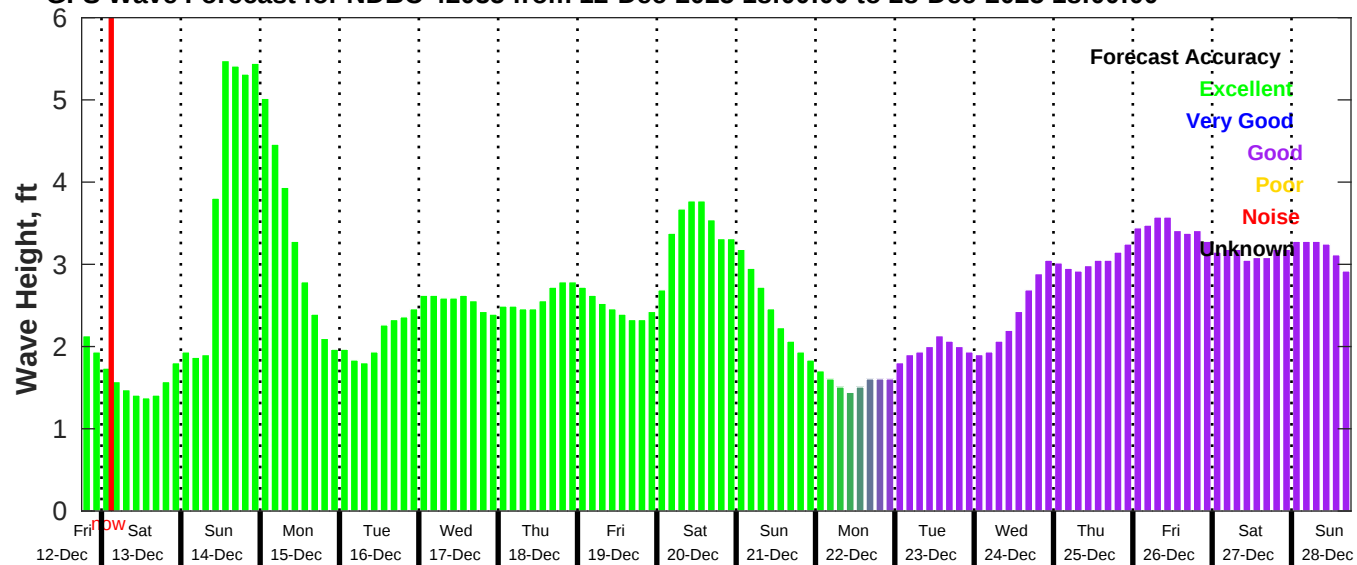
GFS Wave Forecast for NDBC 42035 from 12-Dec-2025 18:00:00 to 28-Dec-2025 18:00:00
