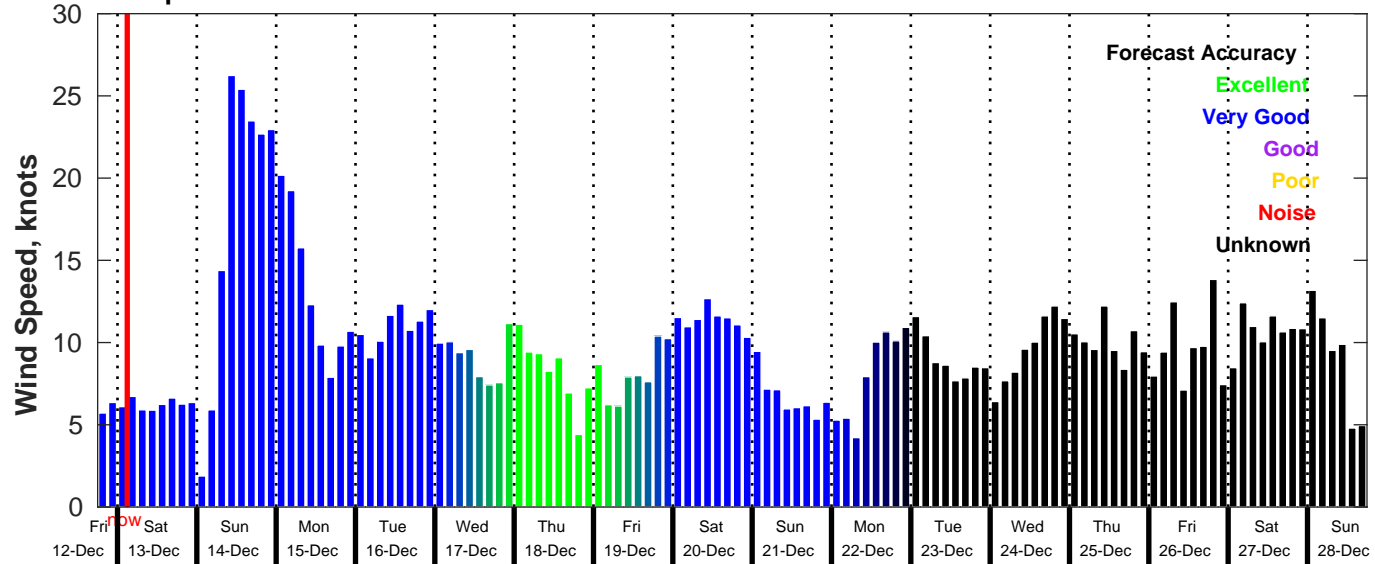
GFS Wind Speed Forecast for NDBC 42035 from 12-Dec-2025 18:00:00 to 28-Dec-2025 18:00:00
