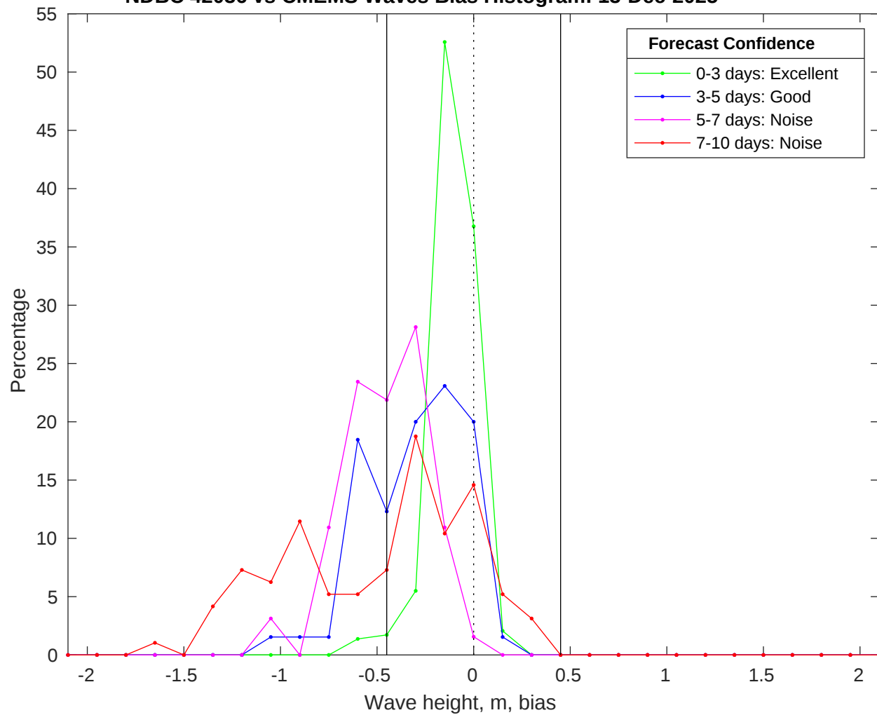
NDBC 42036 vs CMEMS Waves Bias Histogram: 13-Dec-2025
