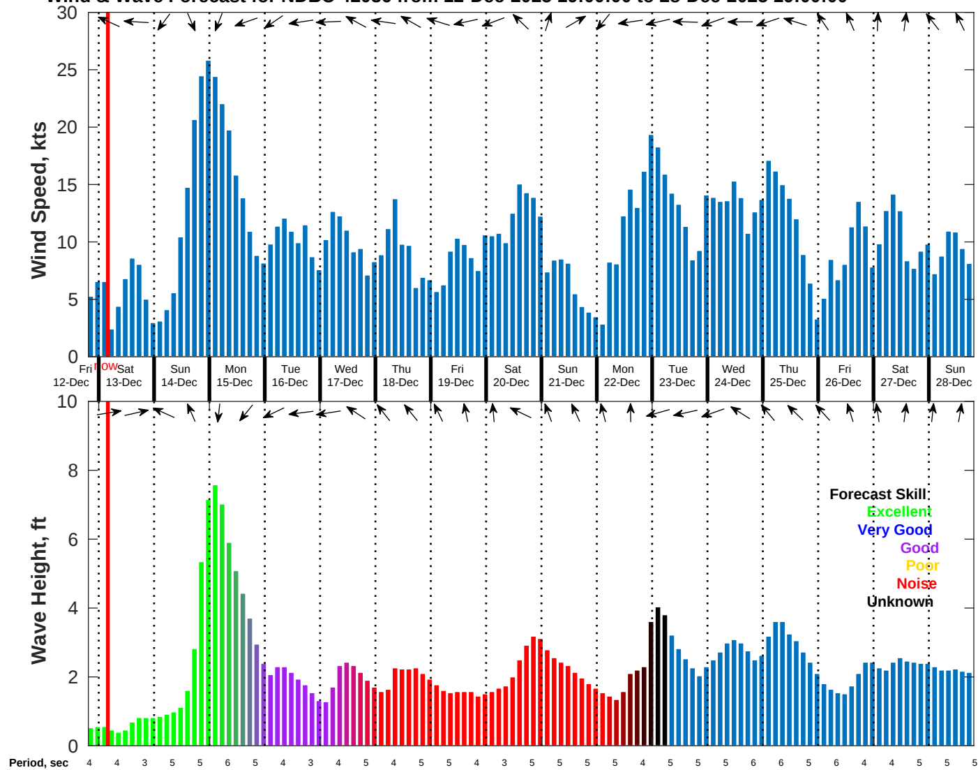
Wind & Wave Forecast for NDBC 42036 from 12-Dec-2025 19:00:00 to 28-Dec-2025 19:00:00
