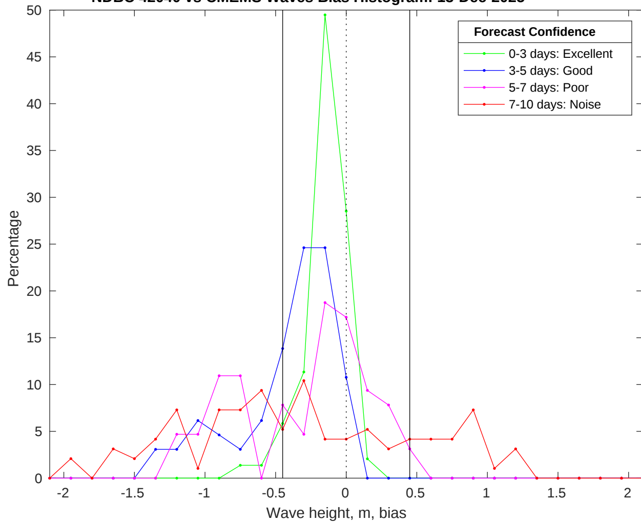
NDBC 42040 vs CMEMS Waves Bias Histogram: 13-Dec-2025
