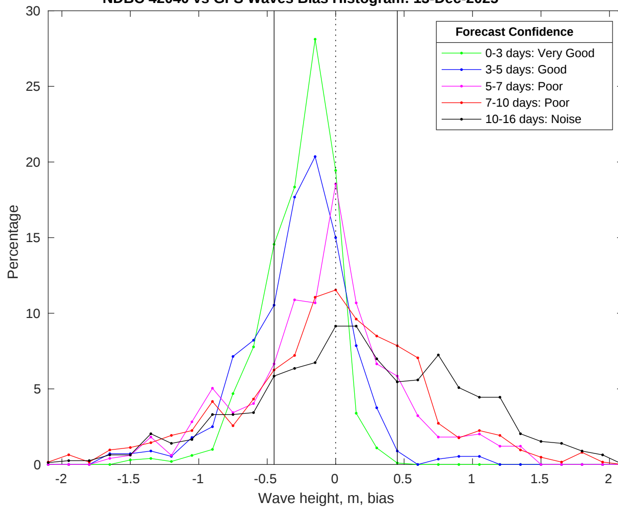
NDBC 42040 vs GFS Waves Bias Histogram: 13-Dec-2025
