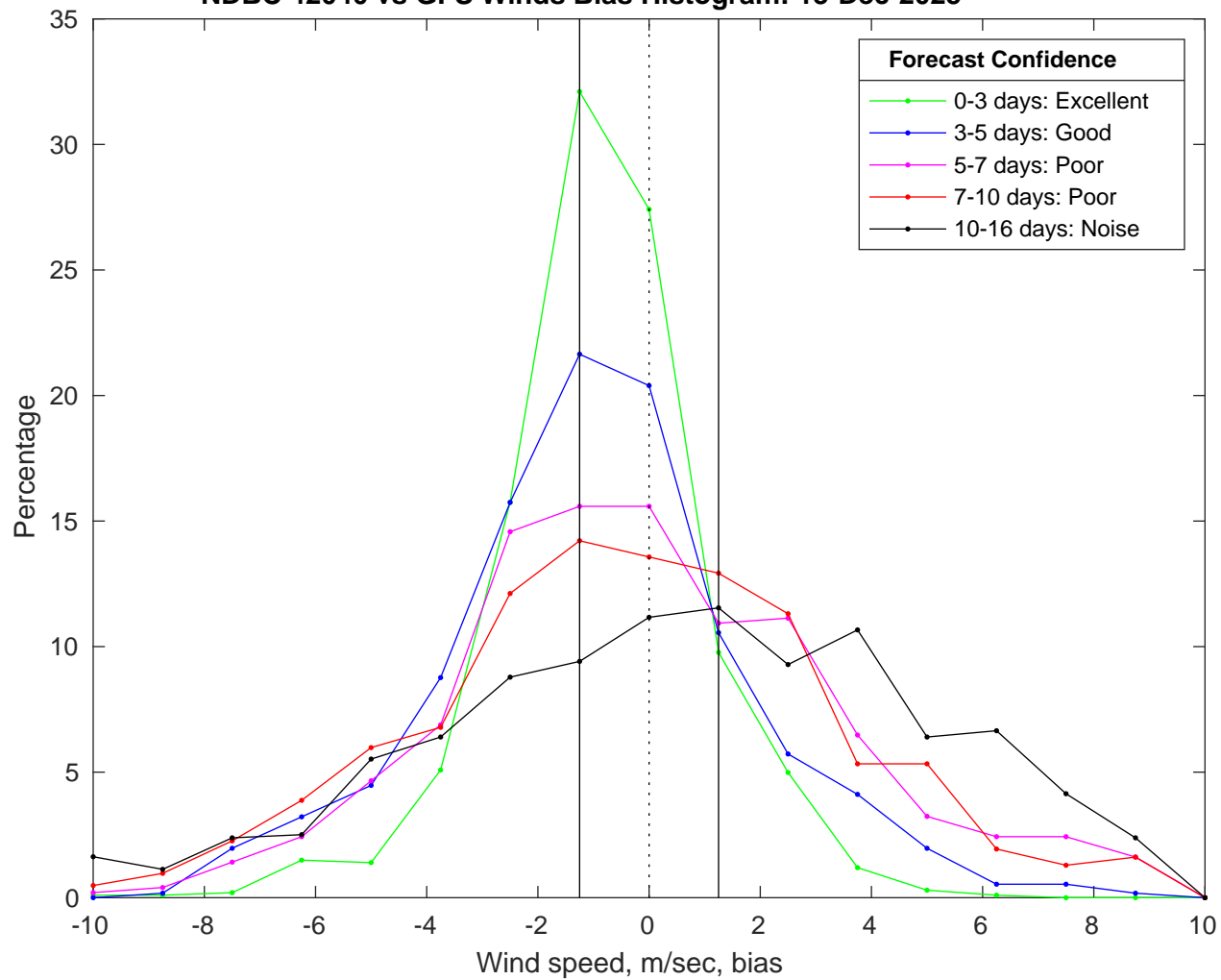
NDBC 42040 vs GFS Winds Bias Histogram: 13-Dec-2025
