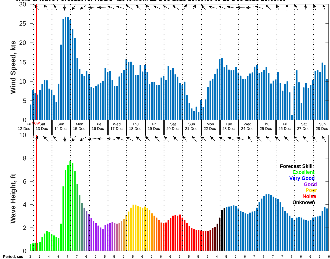
Wind & Wave Forecast for NDBC 42040 from 12-Dec-2025 19:00:00 to 28-Dec-2025 19:00:00
