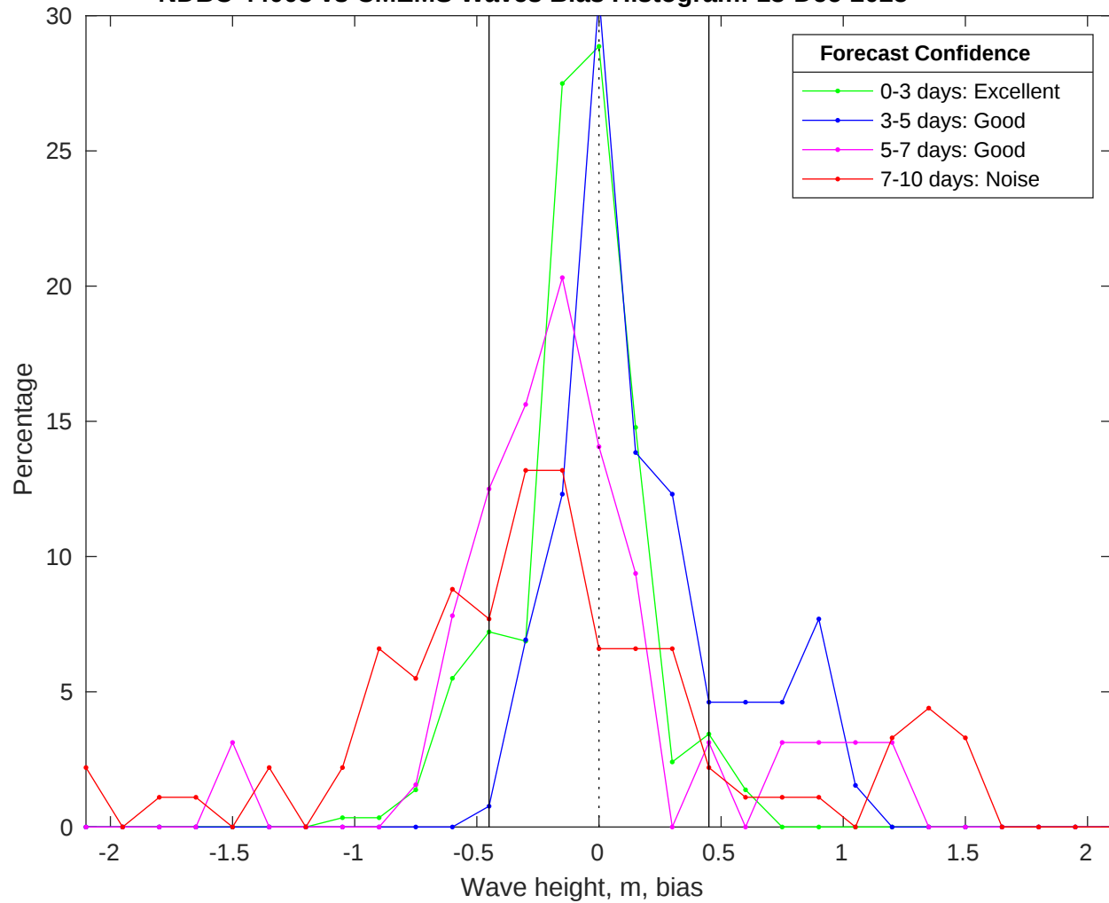
NDBC 44008 vs CMEMS Waves Bias Histogram: 13-Dec-2025
