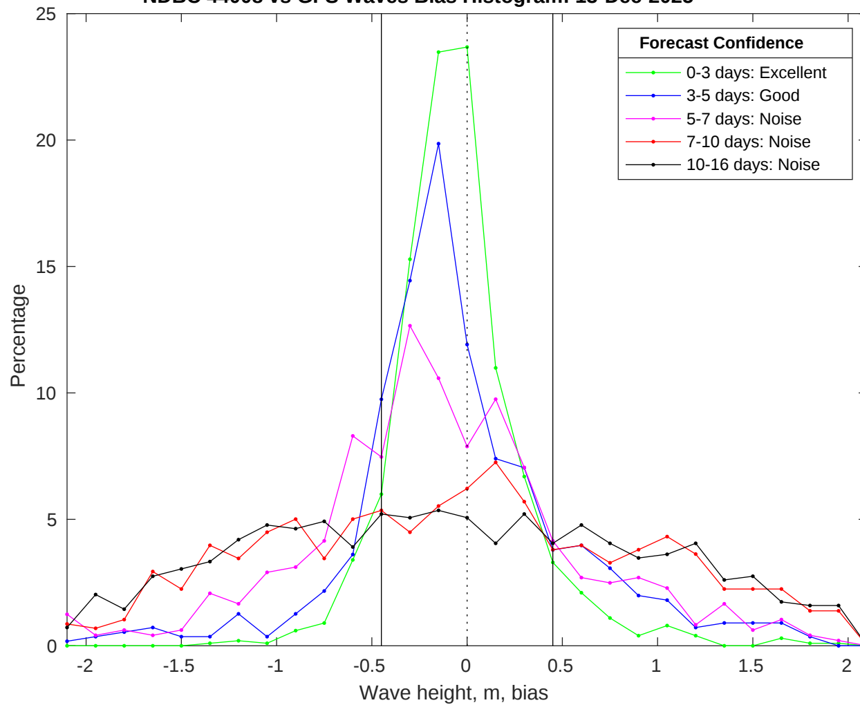
NDBC 44008 vs GFS Waves Bias Histogram: 13-Dec-2025
