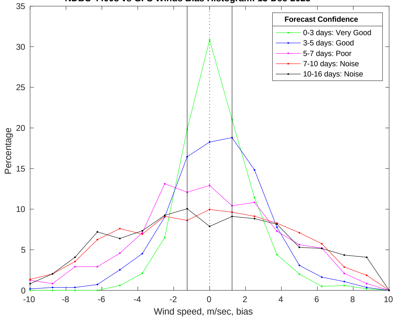
NDBC 44008 vs GFS Winds Bias Histogram: 13-Dec-2025
