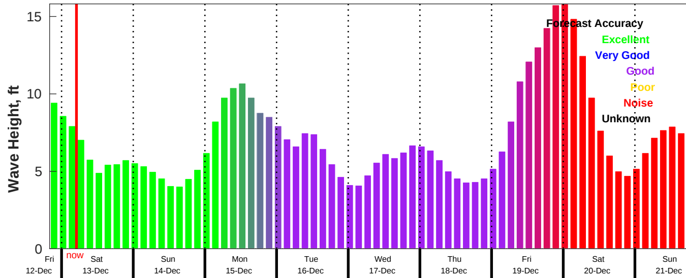
CEMS Wave Forecast for NDBC 44008 from 12-Dec-2025 20:00:00 to 21-Dec-2025 20:00:00
