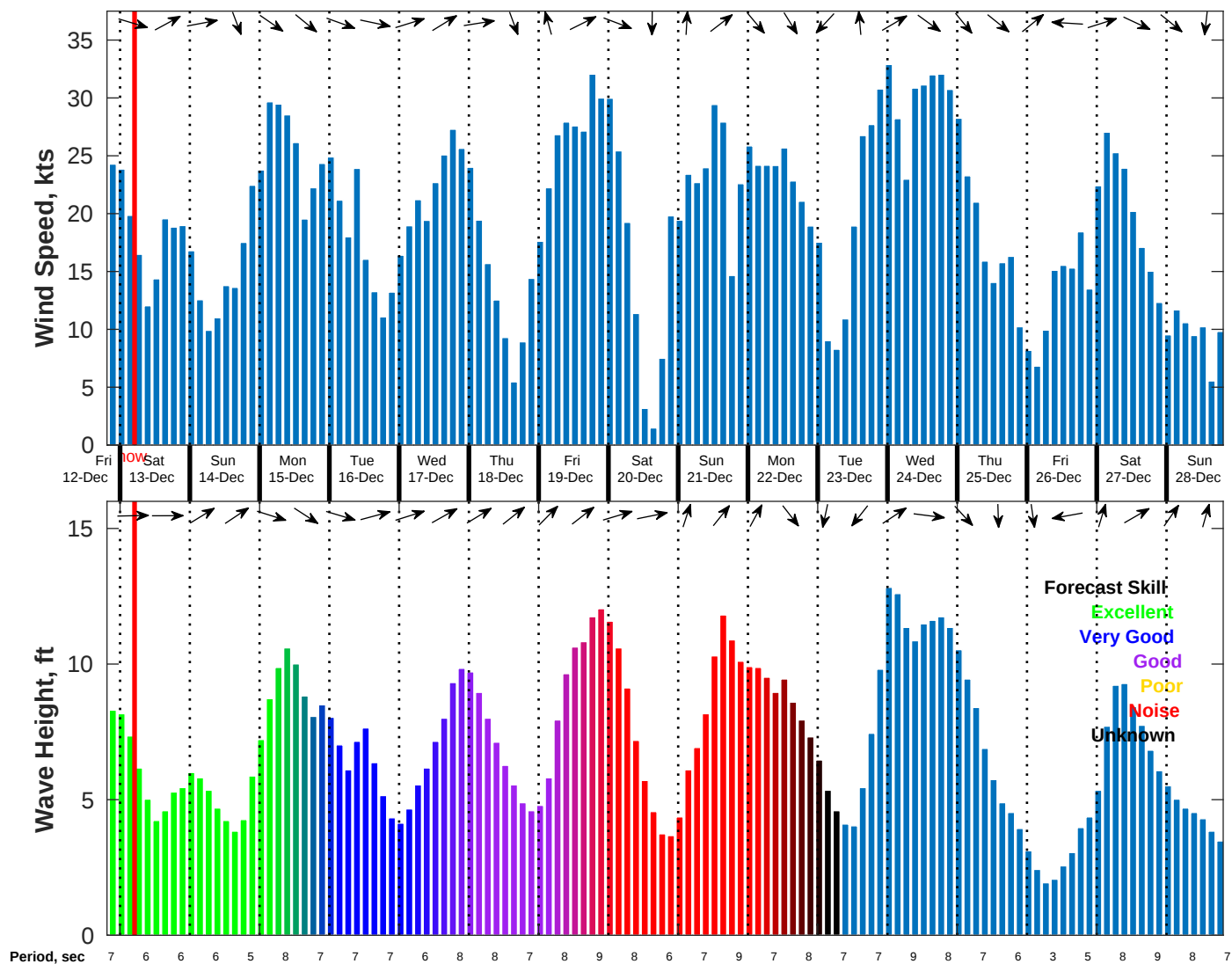
Wind & Wave Forecast for NDBC 44008 from 12-Dec-2025 20:00:00 to 28-Dec-2025 20:00:00
