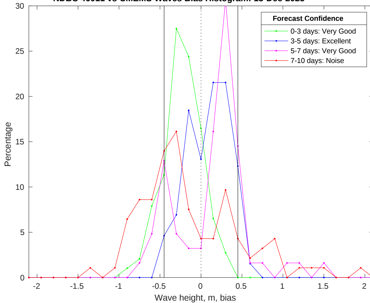
NDBC 46011 vs CMEMS Waves Bias Histogram: 13-Dec-2025
