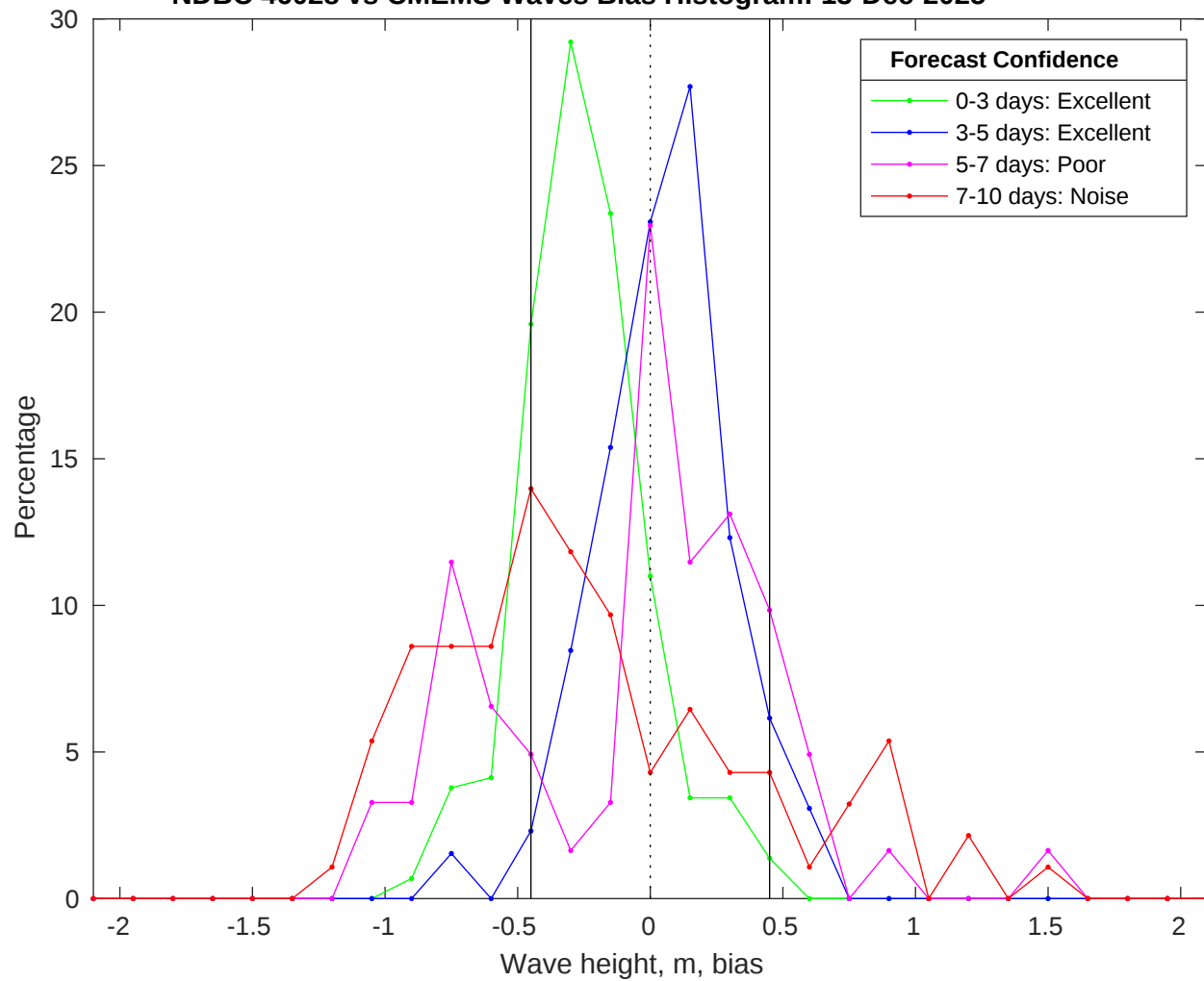
NDBC 46028 vs CMEMS Waves Bias Histogram: 13-Dec-2025
