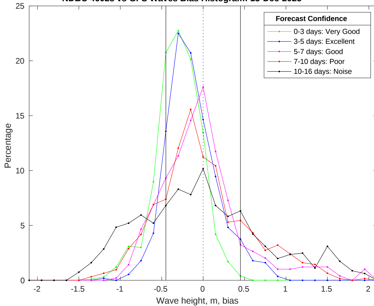
NDBC 46028 vs GFS Waves Bias Histogram: 13-Dec-2025
