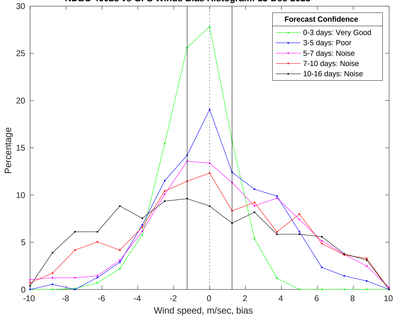
NDBC 46028 vs GFS Winds Bias Histogram: 13-Dec-2025
