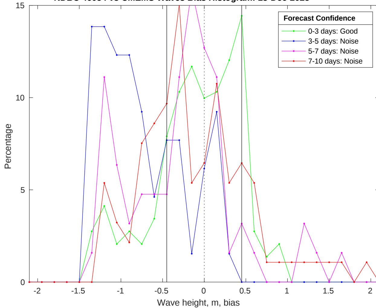
NDBC 46054 vs CMEMS Waves Bias Histogram: 13-Dec-2025
