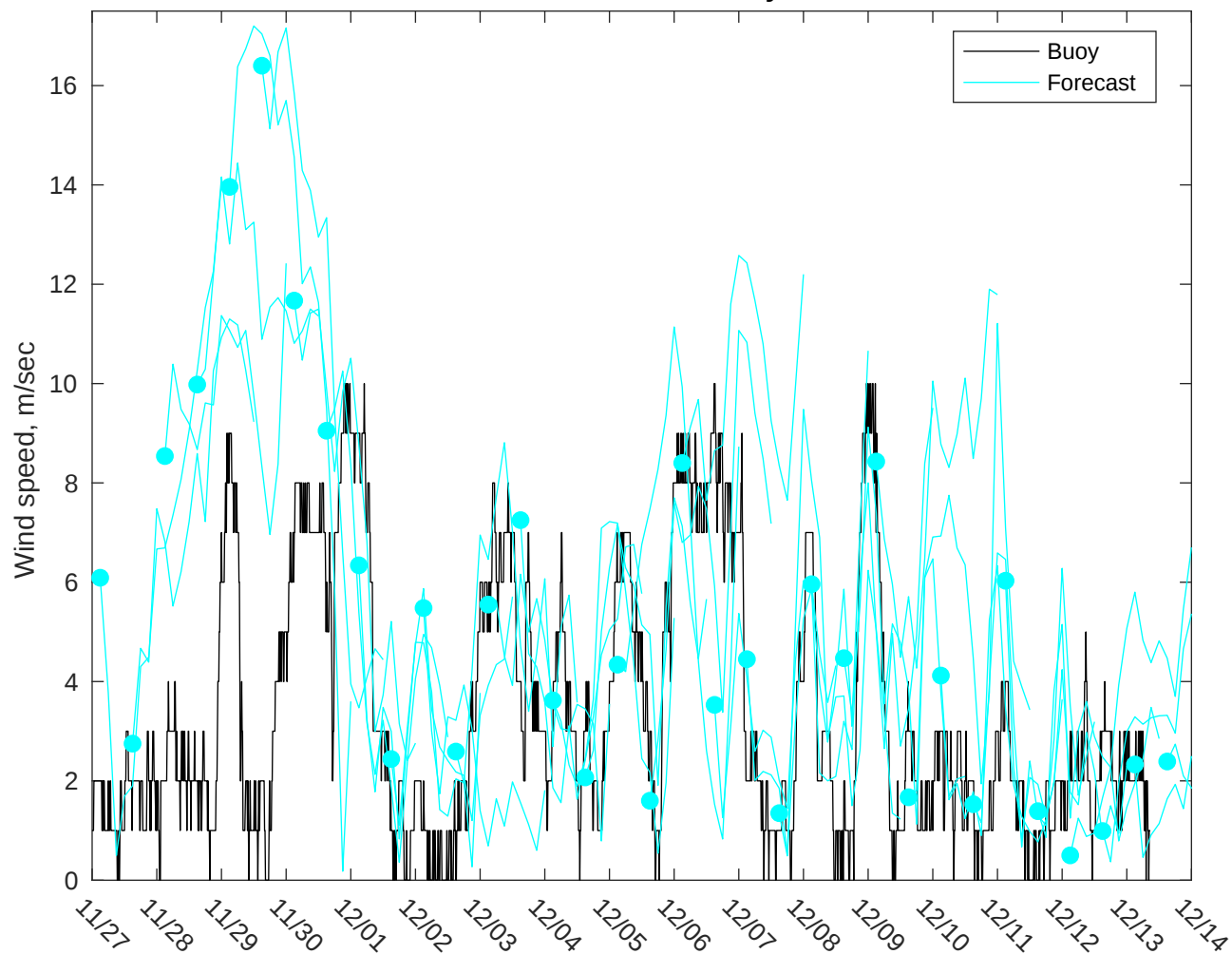
NDBC 46054 vs GFS Winds: 5 to 7 day forecast
