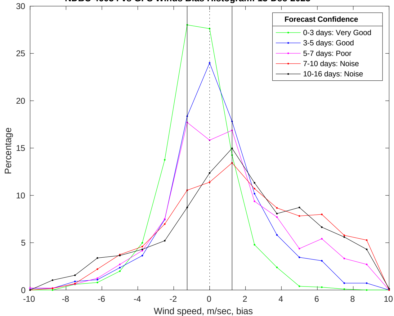
NDBC 46054 vs GFS Winds Bias Histogram: 13-Dec-2025
