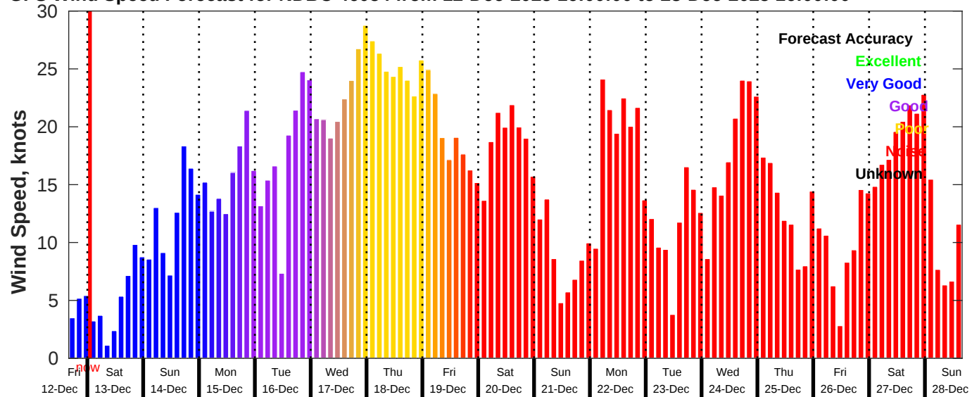
GFS Wind Speed Forecast for NDBC 46054 from 12-Dec-2025 16:00:00 to 28-Dec-2025 16:00:00
