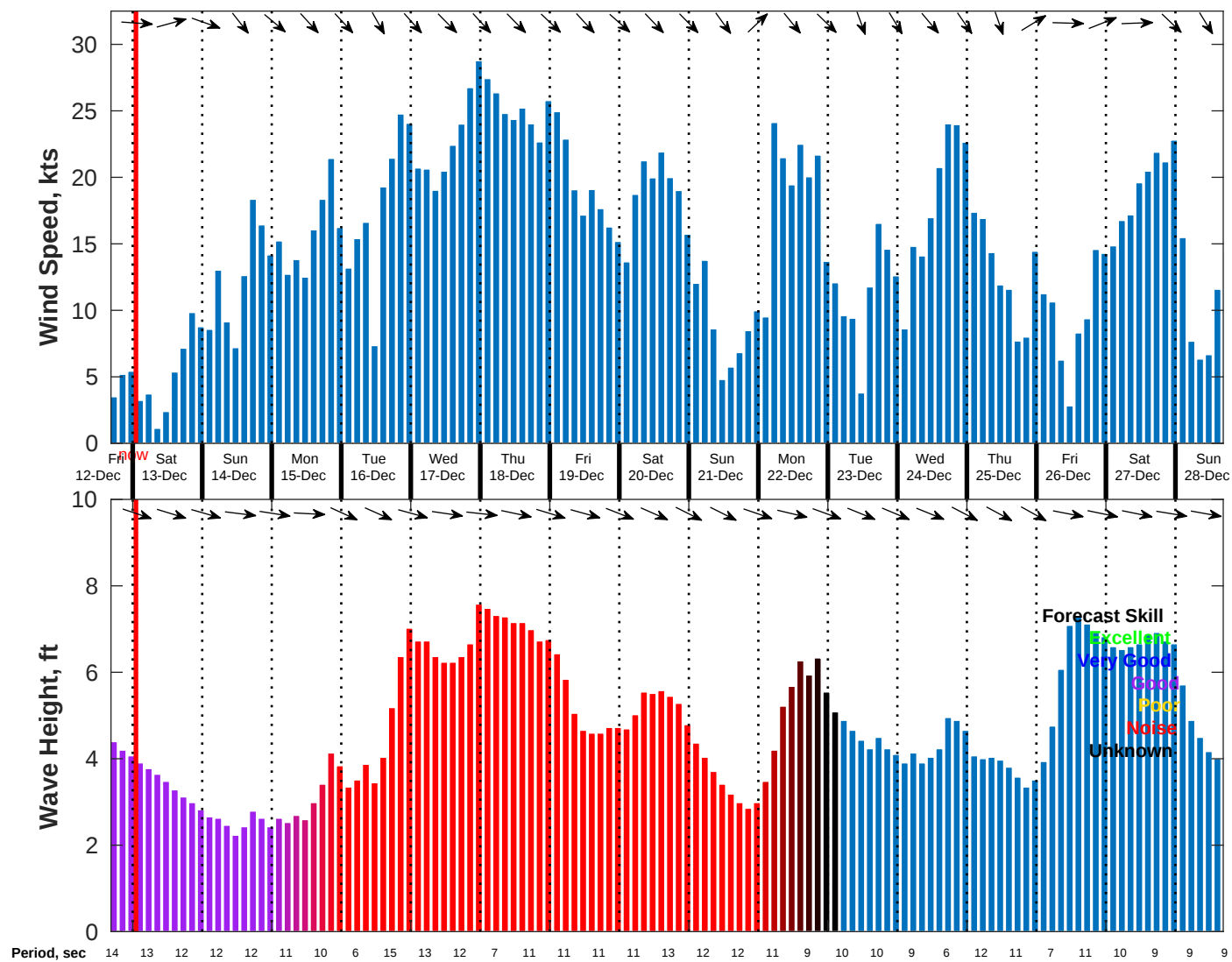
Wind & Wave Forecast for NDBC 46054 from 12-Dec-2025 16:00:00 to 28-Dec-2025 16:00:00
