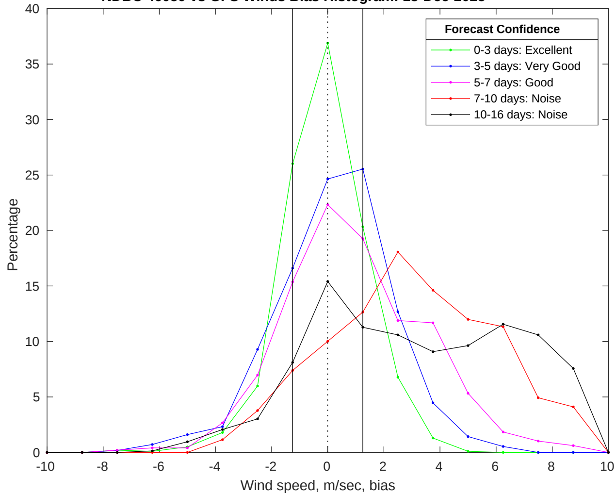
NDBC 46059 vs GFS Winds Bias Histogram: 13-Dec-2025
