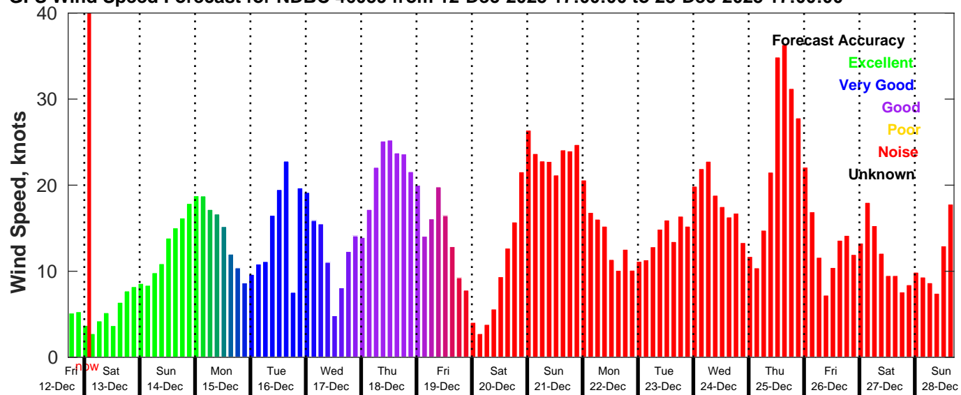
GFS Wind Speed Forecast for NDBC 46059 from 12-Dec-2025 17:00:00 to 28-Dec-2025 17:00:00
