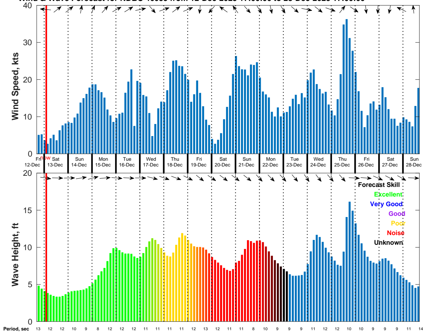
Wind & Wave Forecast for NDBC 46059 from 12-Dec-2025 17:00:00 to 28-Dec-2025 17:00:00
