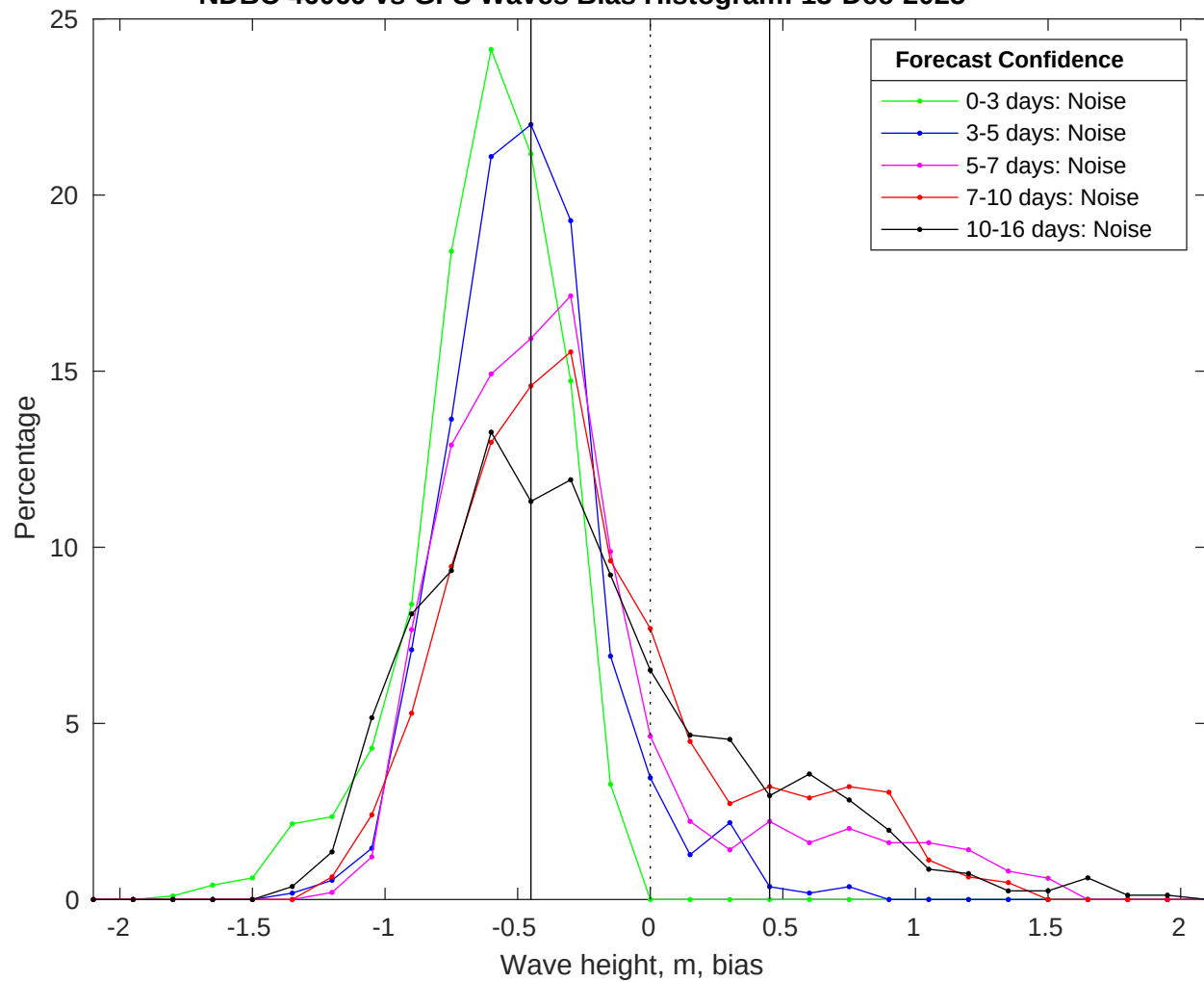
NDBC 46069 vs GFS Waves Bias Histogram: 13-Dec-2025
